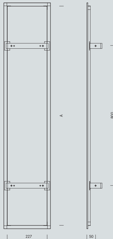
Maßskizze 1 Dimensional drawing 1
