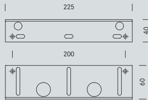
Maßskizze 16 Dimensional drawing 16
