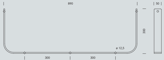
Maßskizze 6 Dimensional drawing 6
