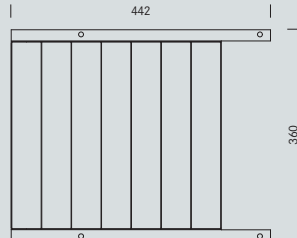
Maßskizze 7 Dimensional drawing 7
