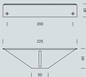
Maßskizze 17 Dimensional drawing 17
