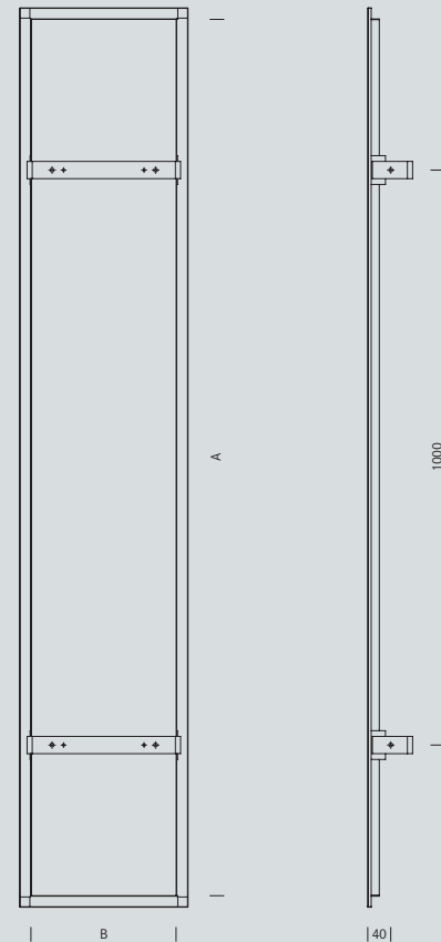
Maßskizze 18 Dimensional drawing 18
