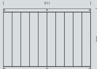
Maßskizze 8 Dimensional drawing 8
