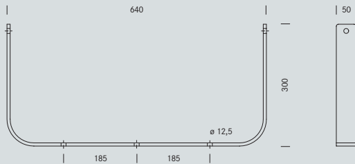
Maßskizze 5 Dimensional drawing 5
