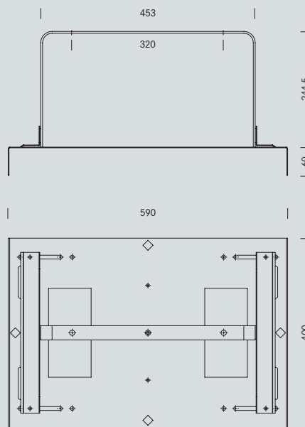
Maßskizze 10 Dimensional drawing 10
